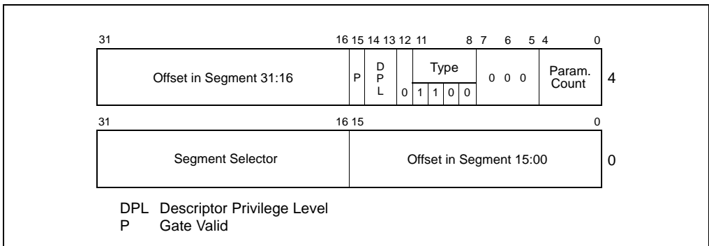
Figure 4-8. Call-Gate Descriptor
