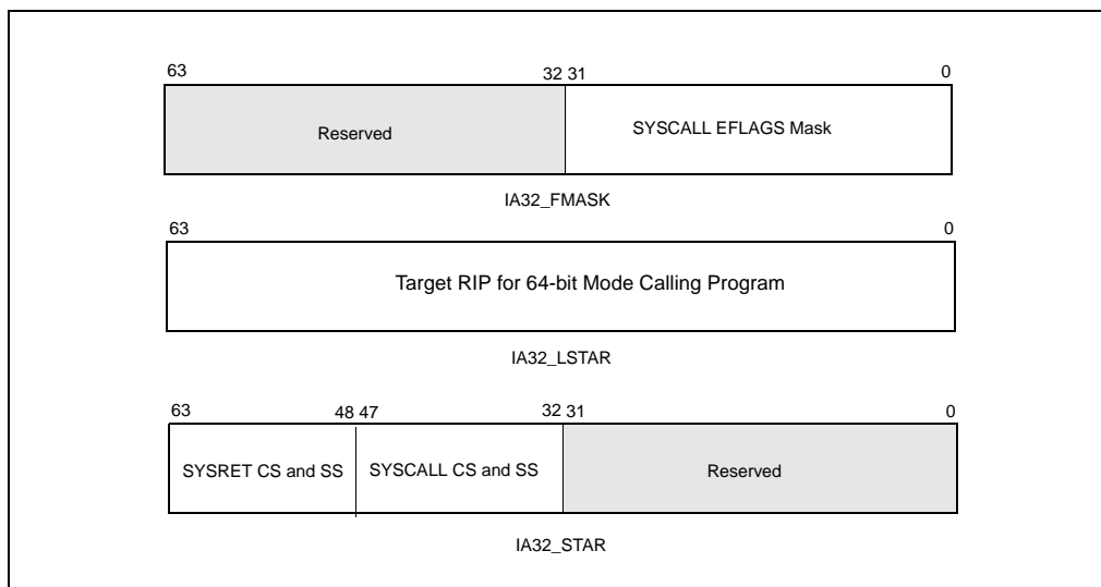
Figure 4-14. MSRs Used by SYSCALL and SYSRET
