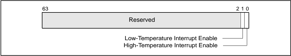
Figure 13-6. IA32_THERM_INTERRUPT MSR
