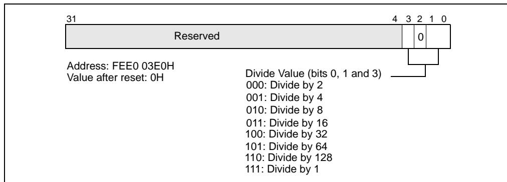
Figure 8-10. Divide Configuration Register
