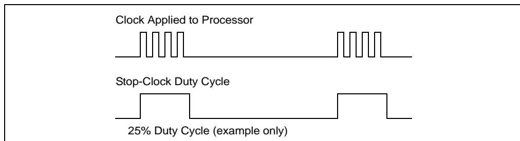
Figure 13-2. Processor Modulation Through Stop-Clock Mechanism
